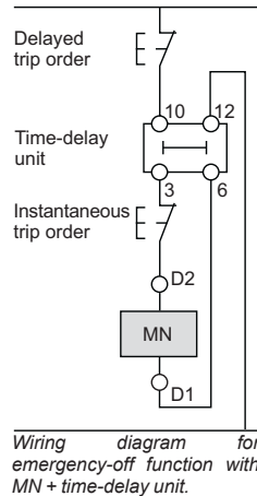
MN release with a time-delay unit.
