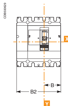
4P
