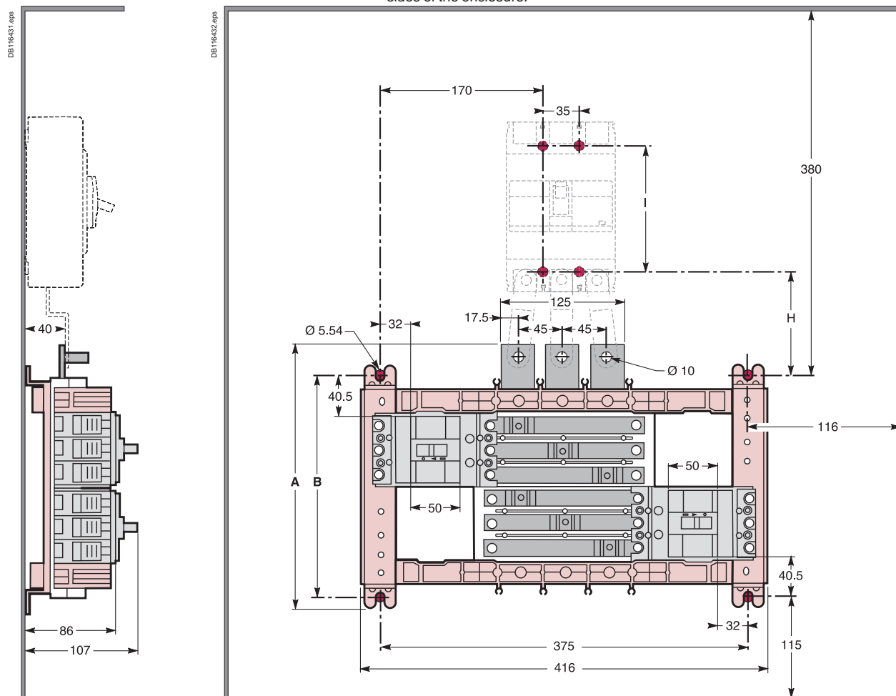
EZB250 - 250 A main busbar rating.
