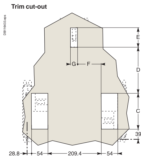
EZB250 - 250 A main busbar rating.
