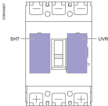
SHT and UVR releases on EZC250.
