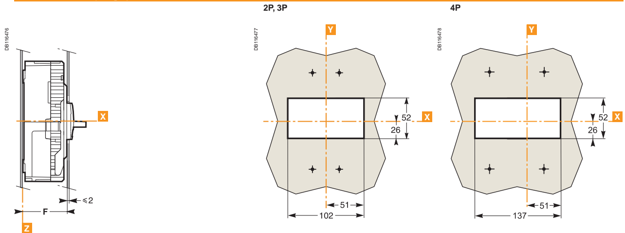
Dimensions (mm)
