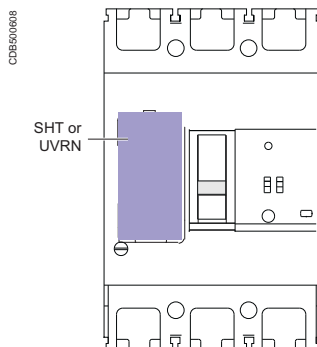
UVRN release on EZCV250.
